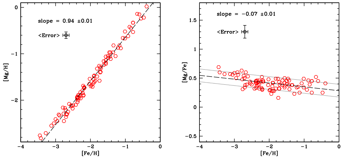
Fig. 17.— These plots are the analogs of Figures 13 and 14 for Mg instead of O. There is a very tight correlation between [Mg/H] and [Fe/H] .
