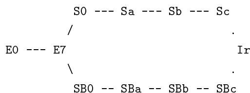
Figure 2.1: Hubble’s ‘tuning-fork’ diagram.
