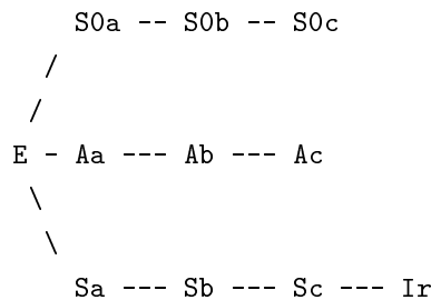
Figure 2.2: van den Berghs’ ‘trident’ diagram.
